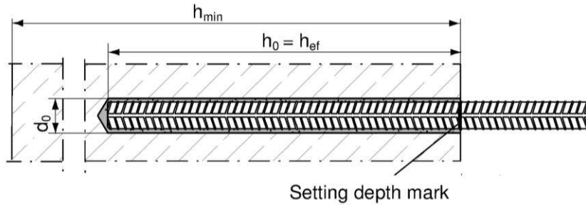
Reinforcing bar
