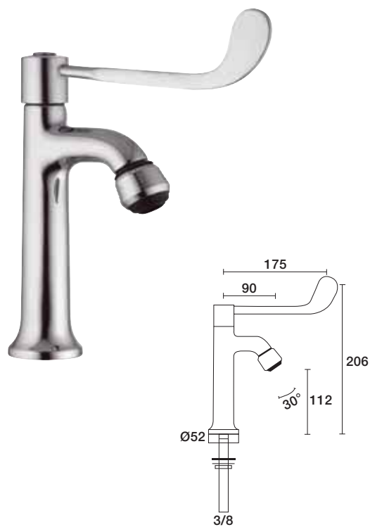
Colonnina bar leva clinica Public bar clinic lever tap
