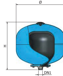
AS 25
