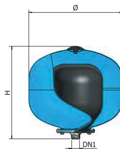
AS 25
