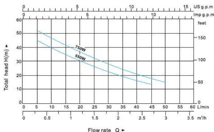
PERFORMANCE CHART AT n=2900 r/min
