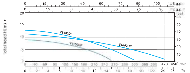
PERFORMANCE CHART AT n=2900 r/min
