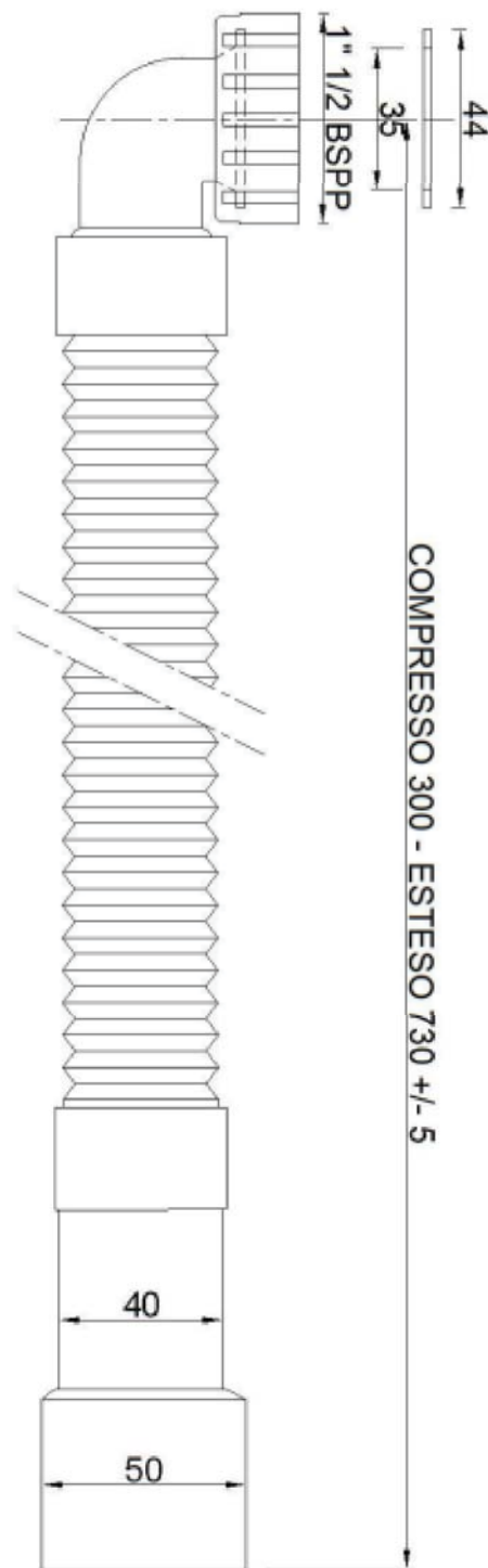
P1000PLCURVA6
